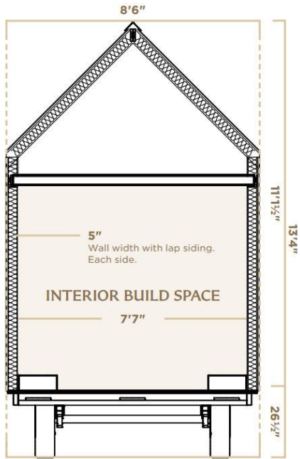
8'6" is the max width allowed by the Department of Transportation (DoT). All measurements approximate. Low-Wider trailer only.
